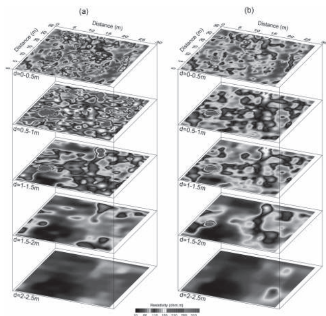
Figure 3 (see color plate): Inversion and sensitivity model depth slices of a) combined form and b) arithmetic mean of arrays (Wenner, Wenner-Schlumberger, dipole-dipole and pole-pole). ABS error values are 3.5% and 3.75%, respectively.
